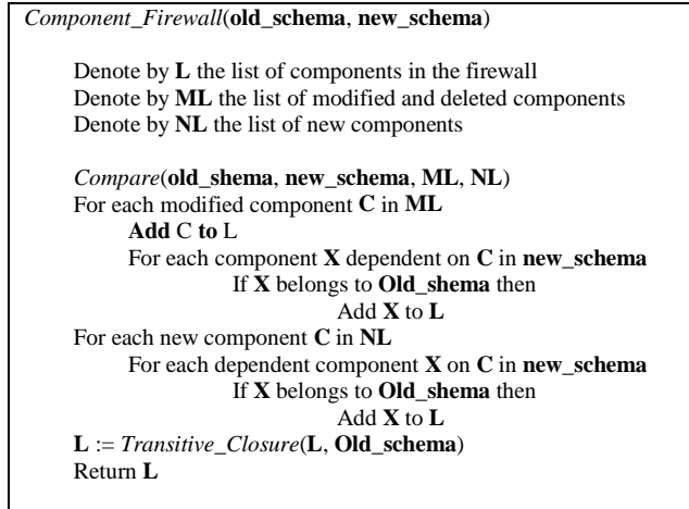
Figure 1 The Component Firewall Algorithm.
