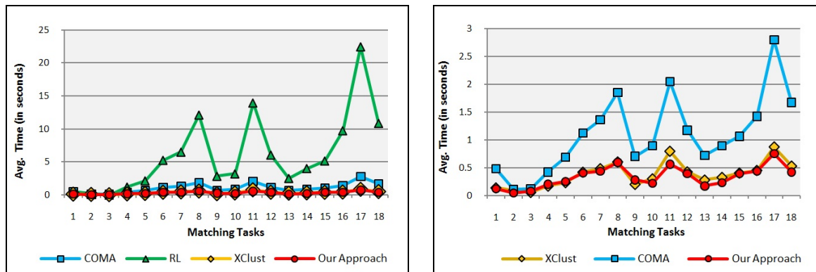
a. Comparison results including Relaxation Labeling .
