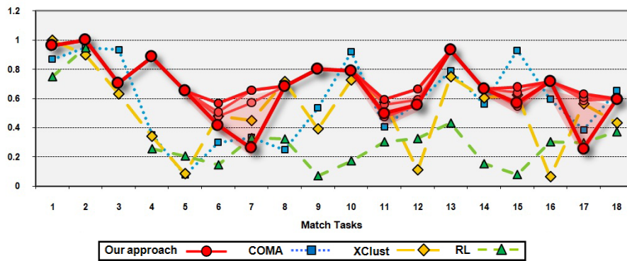
Figure 20. F-Value results, comparing our method with COMA [15], XClust [33] and RL [69].
