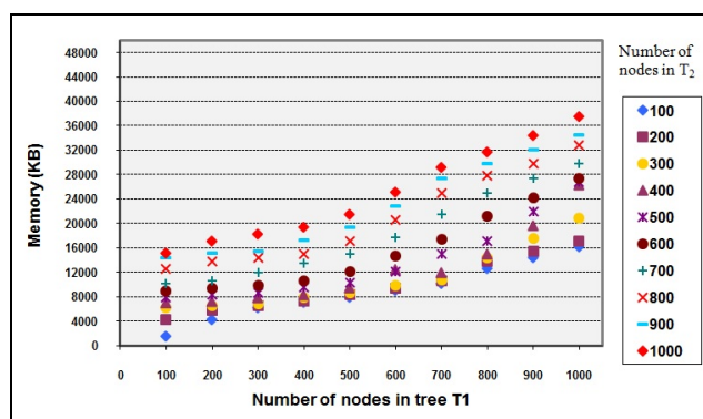
Figure 23. Memory usage.
