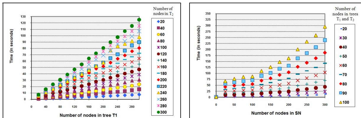
a. Timing analysis with Semantic matcher deactivated. b. Timing analysis with Semantic matcher activated.
