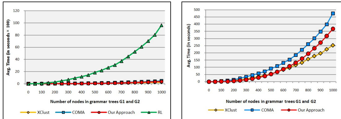
a. Time results, including Relaxation Labeling .
