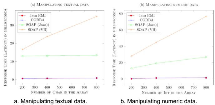
Fig. 3. Comparing SOAP response time, with CORBA [54] and Java RMI [66].
