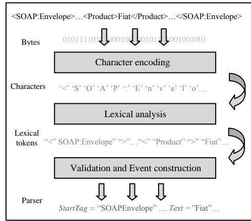
a. Traditional SOAP (XML-based) parsing.
