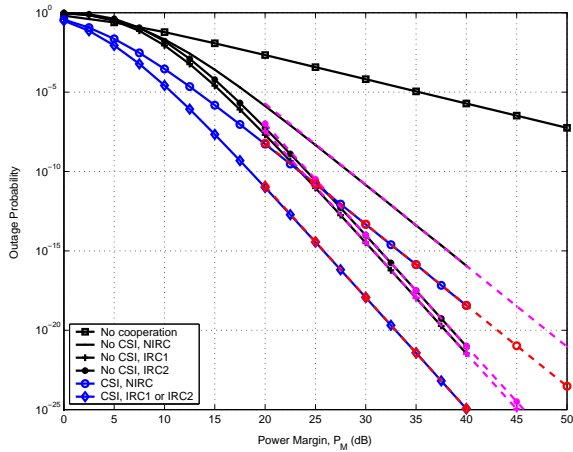
Fig. 3. Performance for (d_{0,1}, d_{1,3}) = (1, 2.5) km and (d_{0,2}, d_{2,3}) = (2.5, 1) km. Solid and dashed lines correspond to the exact outage probabilities and asymptotic bounds, respectively.
