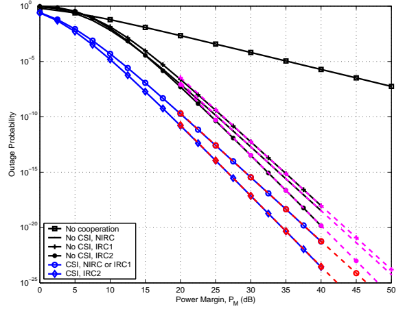
Fig. 4. Performance for (d_{0,1}, d_{1,3}) = (1.8, 1.2) km and (d_{0,2}, d_{2,3}) = (2, 2.7) km. Solid and dashed lines correspond to the exact outage probabilities and asymptotic bounds, respectively.
