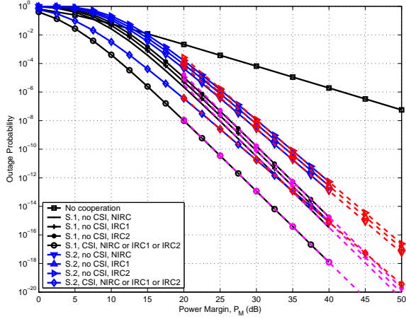
Fig. 2. Performance for setup S.1: (d_{0,1}, d_{1,3}) = (0.8, 2.7) km and (d_{0,2}, d_{2,3}) = (1.2, 2.5) km and for setup S.2: (d_{0,1}, d_{1,3}) = (3, 2) km and (d_{0,2}, d_{2,3}) = (4, 1) km. Solid and dashed lines correspond to the exact outage probabilities and asymptotic bounds, respectively.
