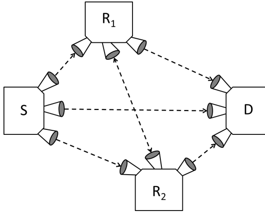
Fig. 1. FSO relay-assisted transmission with two inter-connected relays.
