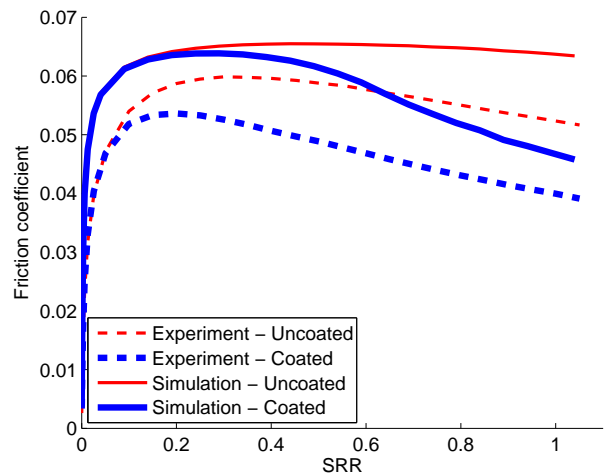
Fig. 7 Friction results at 1.25 GPa, 40°C at 1.0 m/s entrainment speed comparing uncoated and coated specimens in both simulation and experiment.
