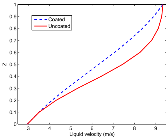
Fig. 11 Lubricant x-velocity profile at the centre of the contact across film thickness. Z=1 is the faster moving surface (ball) and Z=0 is the slower moving surface (disk).
