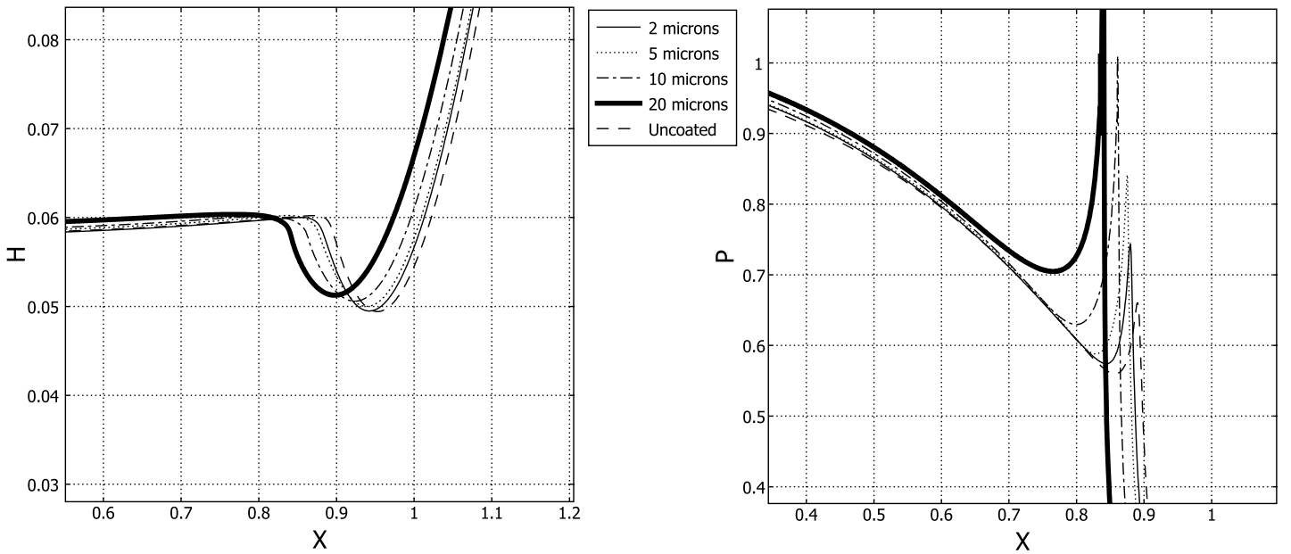
Fig. 3 Effect of DLC coating thickness on the dimensionless film thickness (left) and pressure (right) distribution of a typical EHL line contact (Zoom on Figure 2).
