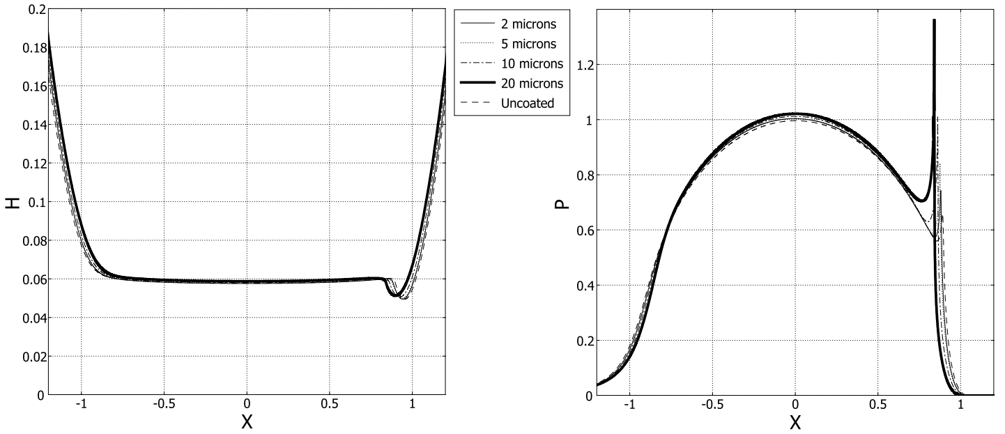
Fig. 2 Effect of DLC coating thickness on the dimensionless film thickness (left) and pressure (right) distribution of a typical EHL line contact.
