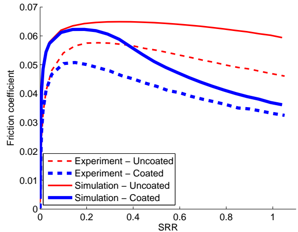
Fig. 6 Friction results at 1.25 GPa, 40°C at 1.611 m/s entrainment speed comparing uncoated and coated specimens in both simulation and experiment.
