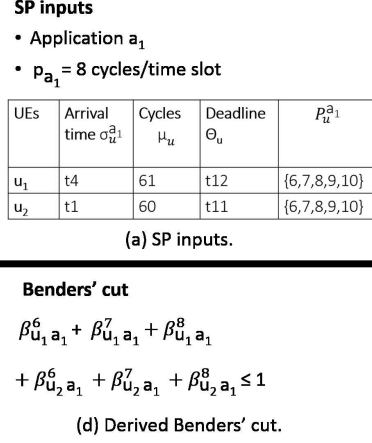
Fig. 3: Benders' cut insights.
