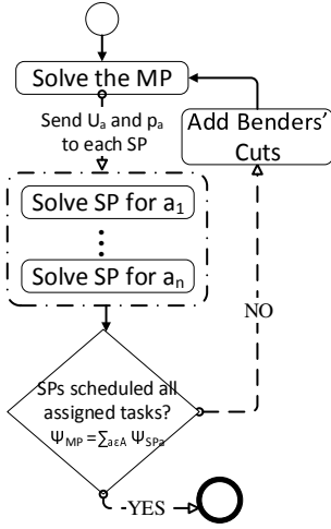
Fig. 2: DTOS-LBBD flowchart.
