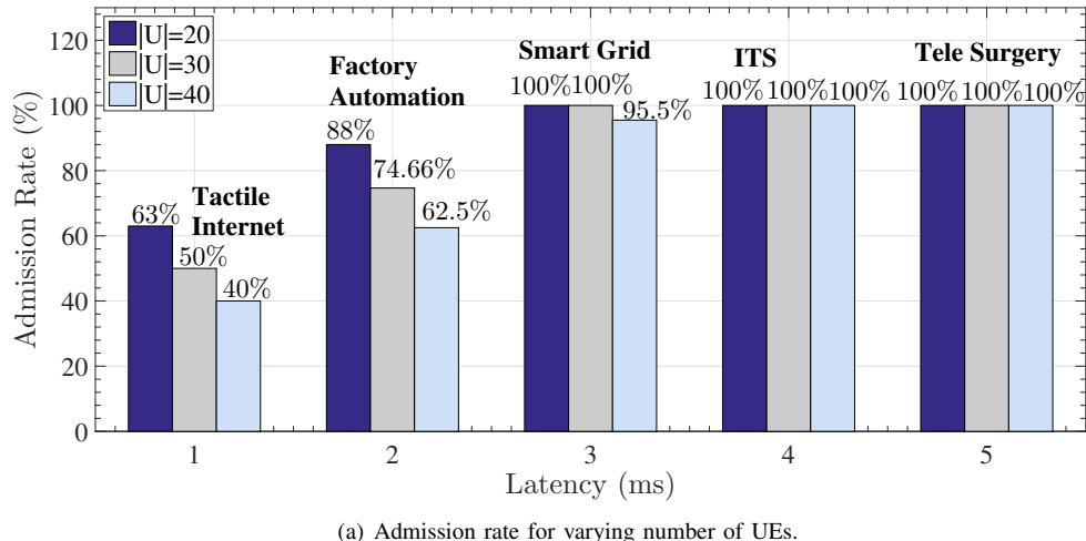
(a) Admission rate for varying number of UEs.
