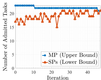
Fig. 4: DTOS-LBBB convergence.
