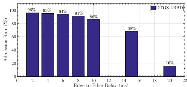
Fig. 6: Admission rate over varying edge-to-edge delay.
